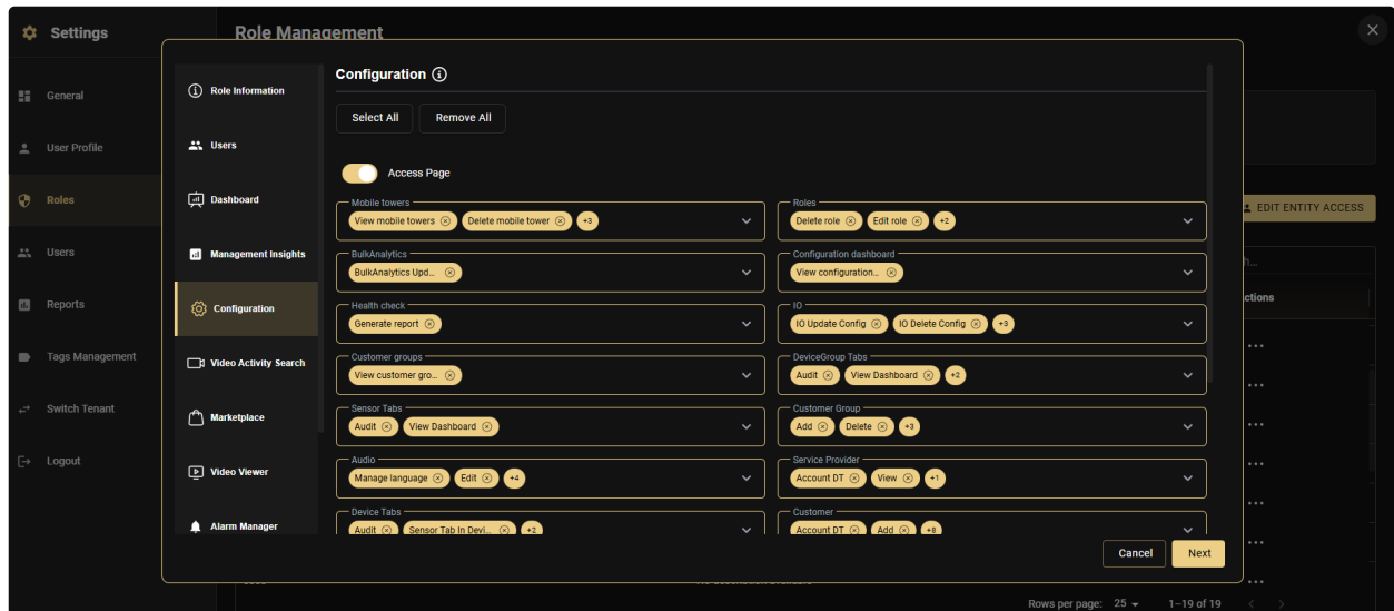
Figure 3.3 — Each module has granular capabilities. The Configuration tab controls adding customers and editing device credentials — Admin only.
